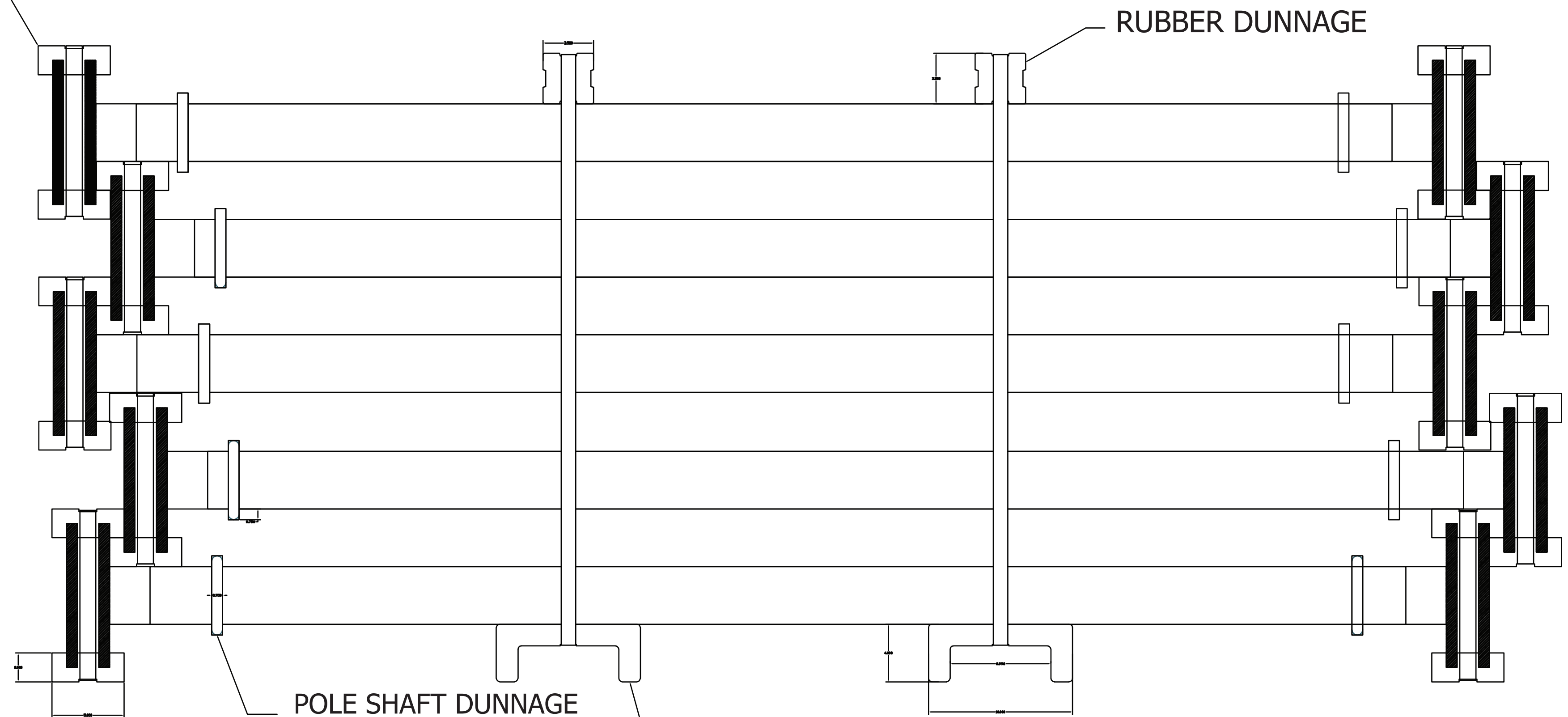
SIDE VIEW OF POLE BUNDLE LAY-OUT
